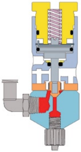
TS5620 Diaphragm Valve
