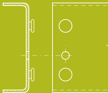
Heavy Rivet beam profile 1830, 2135 & 2440 wide
